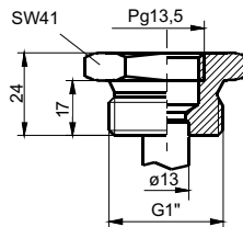
Tank screw fixing 1"
