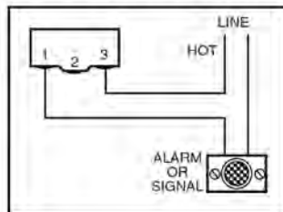
2. Used to sound alarm or light signal when no-flow occurs.
